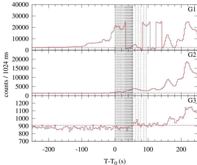
Konus-WIND S2 SOL2004-11-10T02:06 (X2.5) T_0 = 7566.813 s UT (02:06:06.813)
