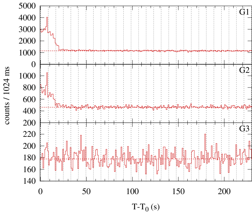
Konus-WIND S2 SOL2004-11-18T14:55 (C3.6) T 0 = 53732.843 s UT (14:55:32.843)
