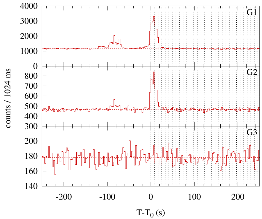
Konus-WIND S2 SOL2004-11-18T14:55 (C3.6) T 0 = 53732.843 s UT (14:55:32.843)
