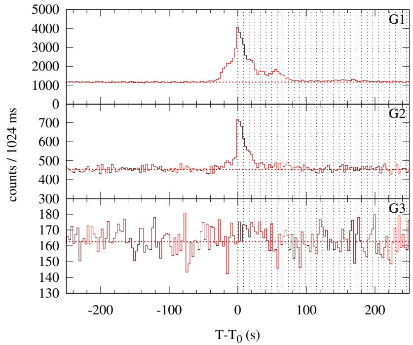
Konus-WIND S2 SOL2004-11-23T15:05 (C6.5) T 0 = 54334.986 s UT (15:05:34.986)
