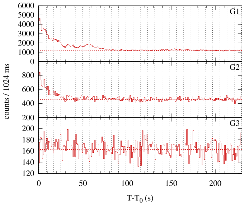
Konus-WIND S2 SOL2004-11-23T15:05 (C6.5) T 0 = 54334.986 s UT (15:05:34.986)
