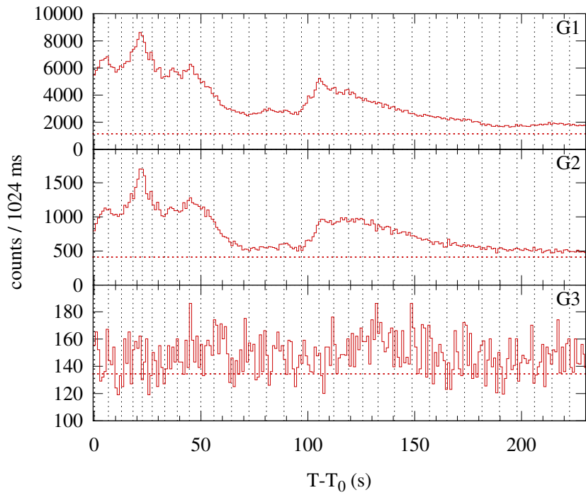
Konus-WIND S2 SOL2004-12-29T16:22 (M2.3) T_0 = 58967.162 s UT (16:22:47.162)
