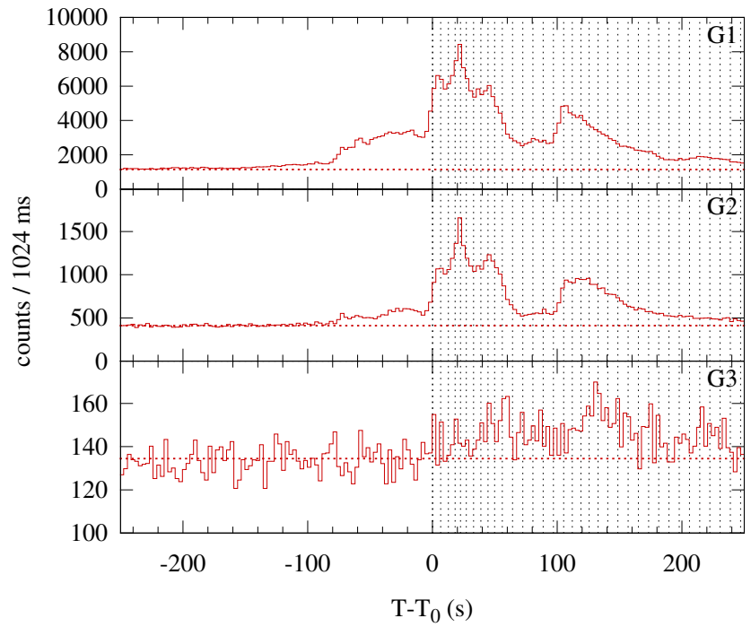
Konus-WIND S2 SOL2004-12-29T16:22 (M2.3) T_0 = 58967.162 s UT (16:22:47.162)
