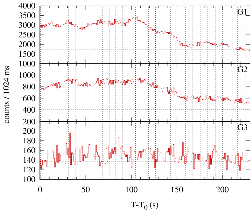
Konus-WIND S2 SOL2004-12-30T22:15 (M4.2) T_0 = 80147.921 s UT (22:15:47.921)
