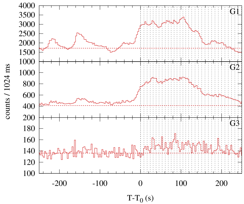
Konus-WIND S2 SOL2004-12-30T22:15 (M4.2) T_0 = 80147.921 s UT (22:15:47.921)
