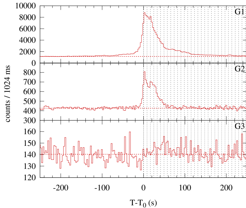
Konus-WIND S2 SOL2005-01-14T13:57 (M1.8) T_0 = 50239.290 s UT (13:57:19.290)
