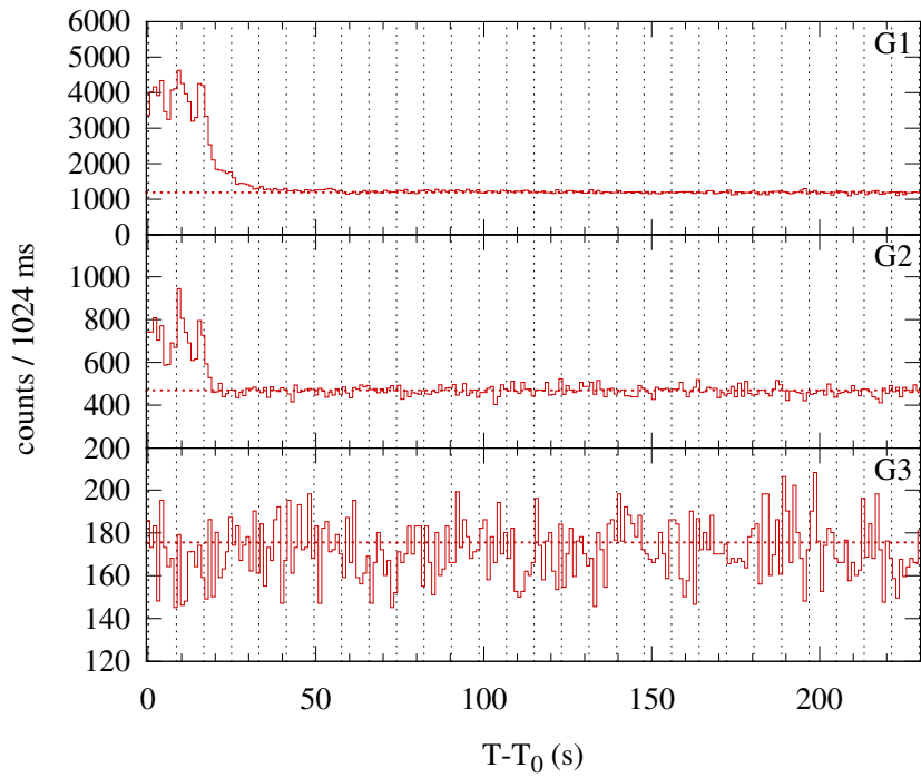
Konus-WIND S2 SOL2005-01-15T19:47 (C3.5) T_0 = 71246.532 s UT (19:47:26.532)
