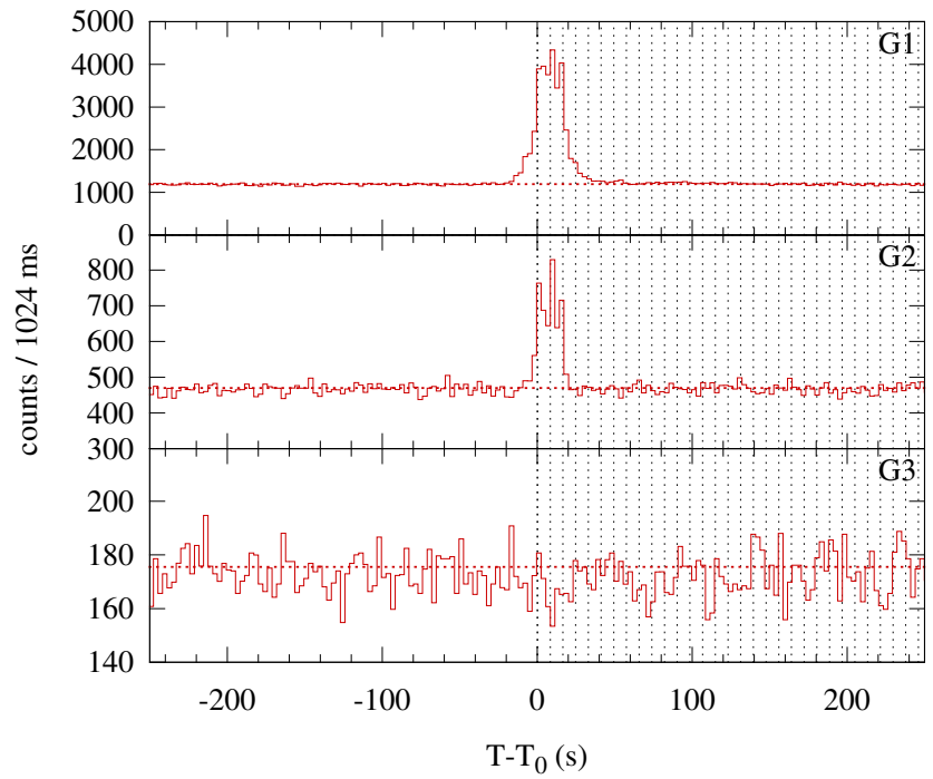
Konus-WIND S2 SOL2005-01-15T19:47 (C3.5) T_0 = 71246.532 s UT (19:47:26.532)
