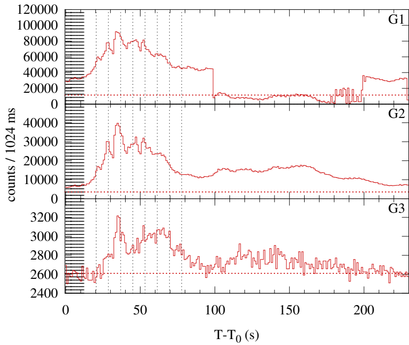
Konus-WIND S2 SOL2005-01-17T09:42 (X3.8) T_0 = 34970.553 s UT (09:42:50.553)
