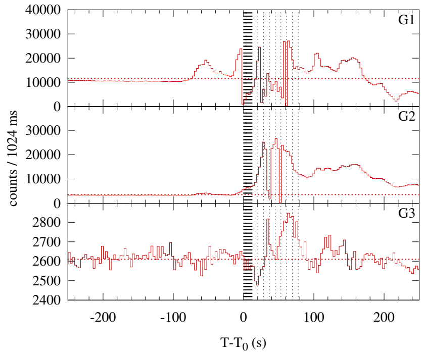
Konus-WIND S2 SOL2005-01-17T09:42 (X3.8) T_0 = 34970.553 s UT (09:42:50.553)
