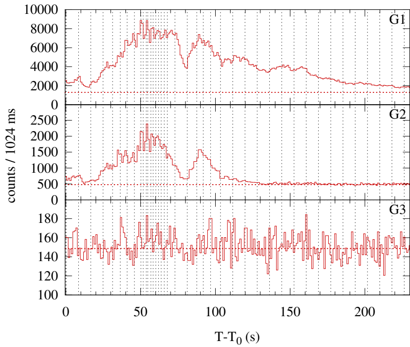
Konus-WIND S2 SOL2005-05-06T03:07 (C9.3) T 0 = 11259.347 s UT (03:07:39.347)
