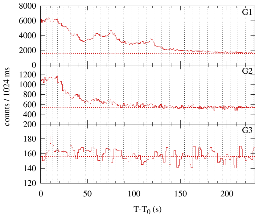
Konus-WIND S2 SOL2005-05-06T11:22 (M1.3) T_0 = 40974.56 s UT (11:22:54.56)
