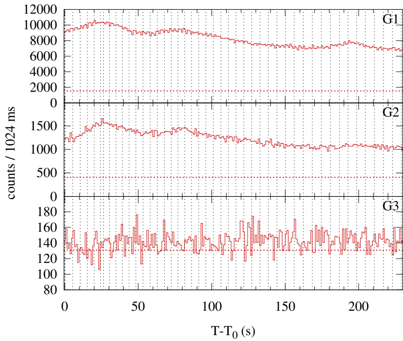
Konus-WIND S2 SOL2005-05-13T16:41 (M8.0) T 0 = 60096.940 s UT (16:41:36.940)
