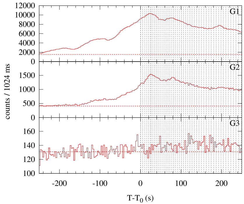
Konus-WIND S2 SOL2005-05-13T16:41 (M8.0) T 0 = 60096.940 s UT (16:41:36.940)
