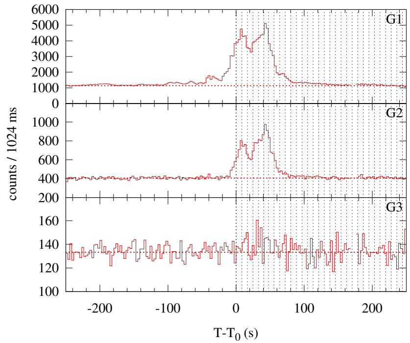
Konus-WIND S2 SOL2005-06-03T04:09 (M1.3) T_0 = 14975.752 s UT (04:09:35.752)
