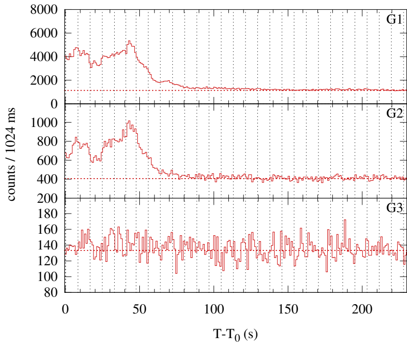
Konus-WIND S2 SOL2005-06-03T04:09 (M1.3) T_0 = 14975.752 s UT (04:09:35.752)
