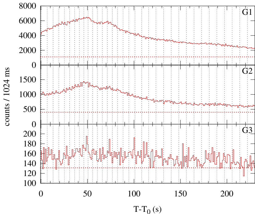
Konus-WIND S2 SOL2005-06-16T20:09 (M4.0) T_0 = 72552.729 s UT (20:09:12.729)
