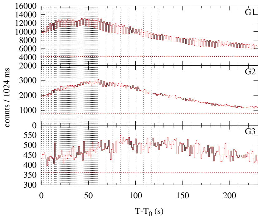
Konus-WIND S1 SOL2005-07-14T10:33 (X1.2) T 0 = 37984.731 s UT (10:33:04.731)
