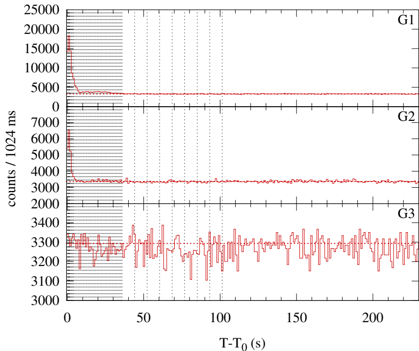
Konus-WIND S2 SOL2005-09-15T04:59 (C2.6) T 0 = 17950.337 s UT (04:59:10.337)
