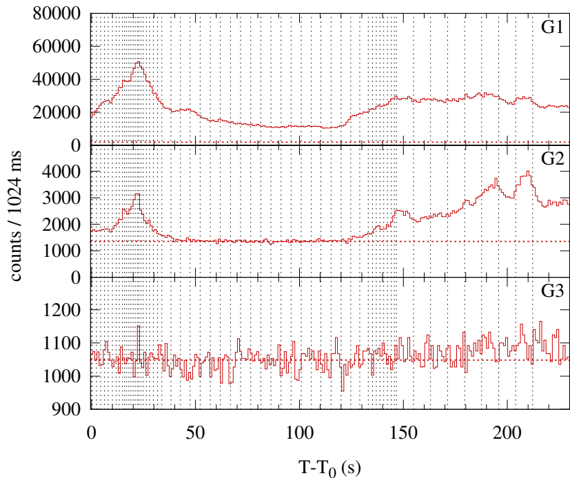
Konus-WIND S2 SOL2005-09-17T06:01 (M9.8) T_0 = 21707.254 s UT (06:01:47.254)
