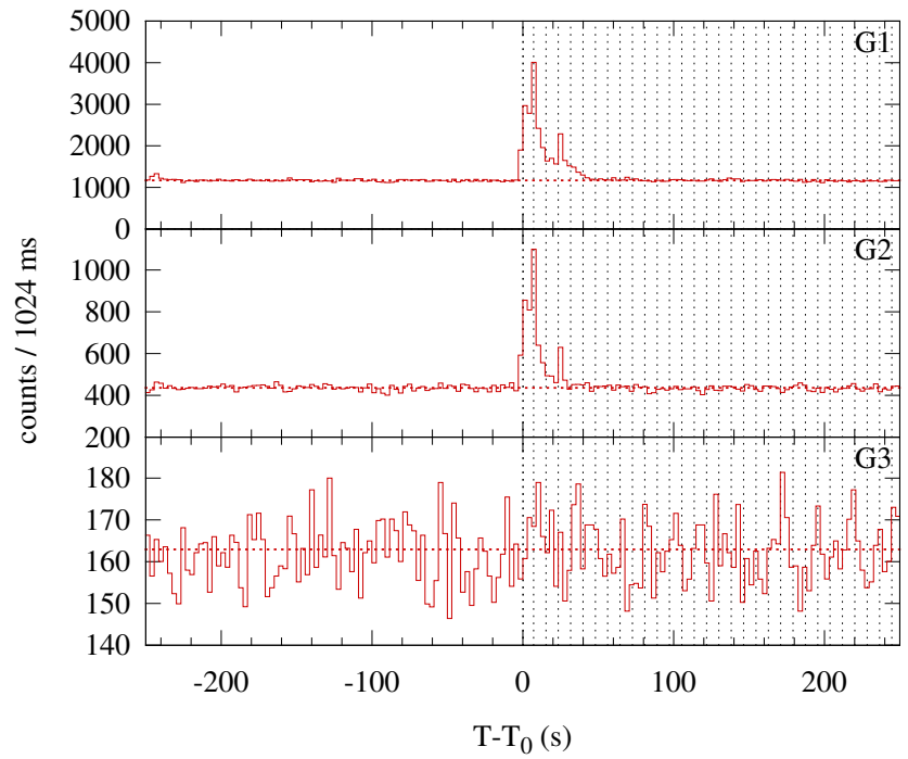
Konus-WIND S2 SOL2006-07-07T00:18 (C2.6) T 0 = 1126.865 s UT (00:18:46.865)
