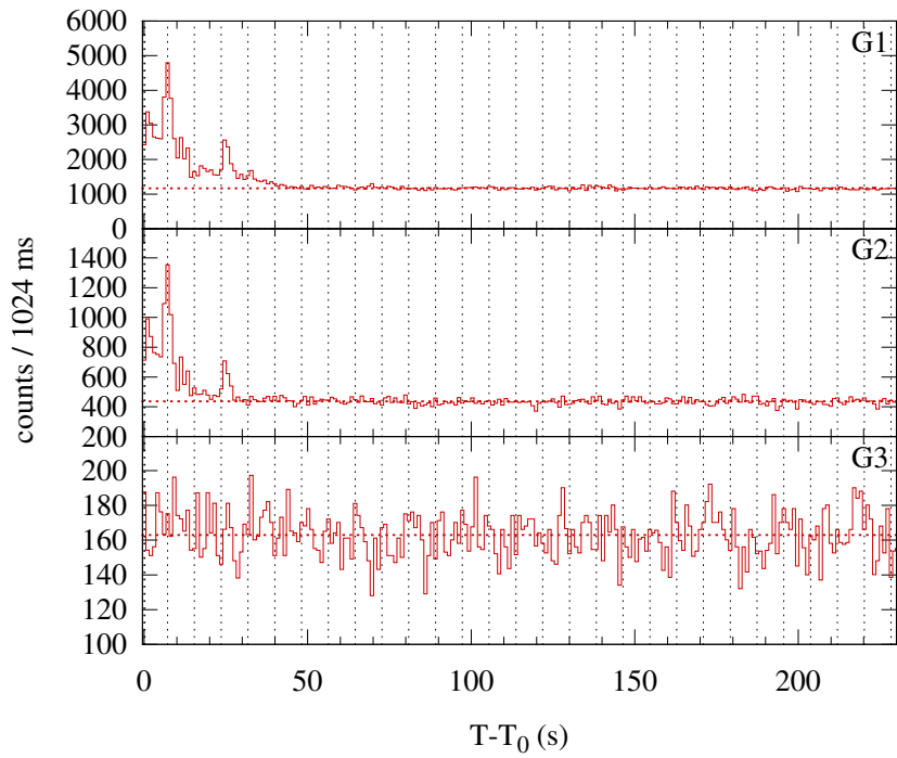
Konus-WIND S2 SOL2006-07-07T00:18 (C2.6) T 0 = 1126.865 s UT (00:18:46.865)
