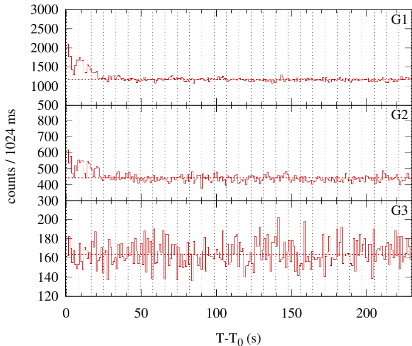
Konus-WIND S2 SOL2006-07-07T04:56 (B2.2) T_0 = 17803.190 s UT (04:56:43.190)
