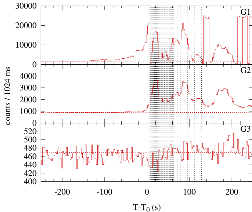
Konus-WIND S2 SOL2006-12-14T22:07 (X1.5) T_0 = 79657.803 s UT (22:07:37.803)
