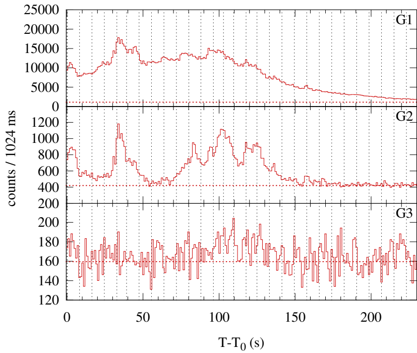
Konus-WIND S2 SOL2007-06-04T05:11 (M8.9) T 0 = 18671.428 s UT (05:11:11.428)
