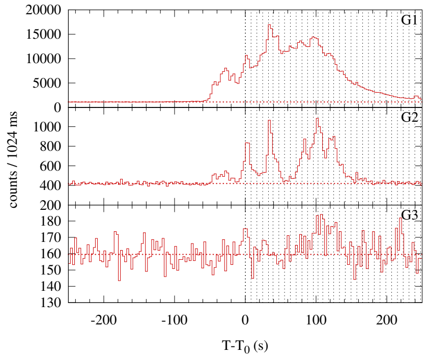
Konus-WIND S2 SOL2007-06-04T05:11 (M8.9) T 0 = 18671.428 s UT (05:11:11.428)
