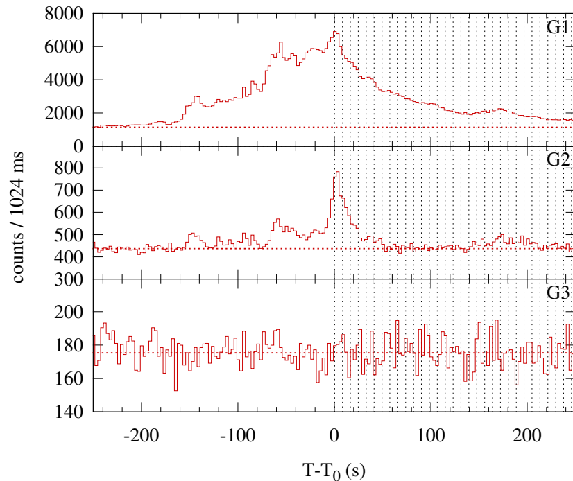
Konus-WIND S2 SOL2010-02-07T02:33 (M6.4) T_0 = 9184.736 s UT (02:33:04.736)
