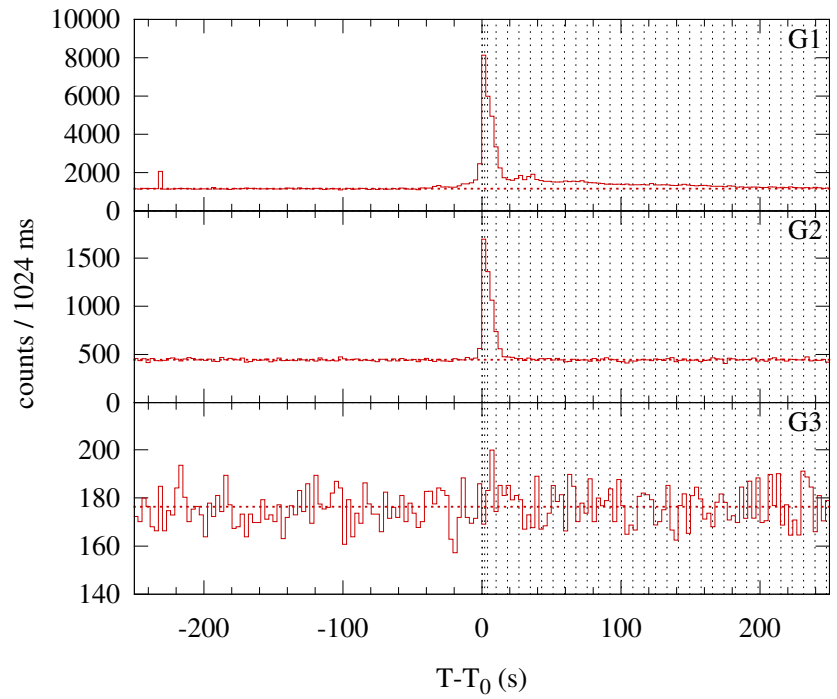
Konus-WIND S2 SOL2010-02-08T13:44 (M2.0) T 0 = 49443.619 s UT (13:44:03.619)
