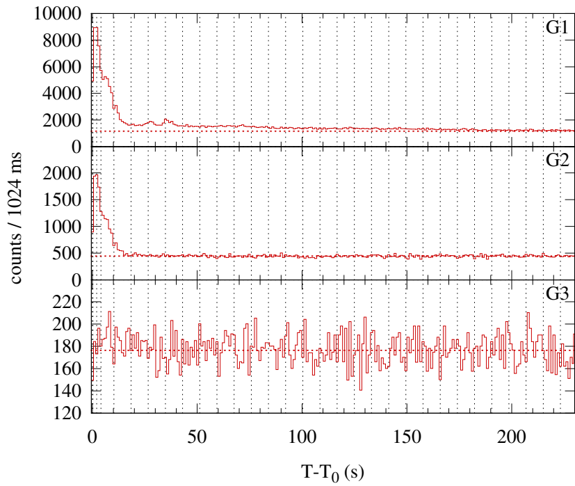
Konus-WIND S2 SOL2010-02-08T13:44 (M2.0) T 0 = 49443.619 s UT (13:44:03.619)
