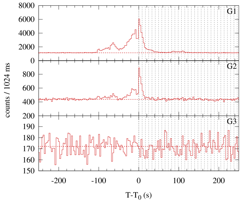
Konus-WIND S2 SOL2010-02-12T07:23 (C7.9) T_0 = 26597.710 s UT (07:23:17.710)
