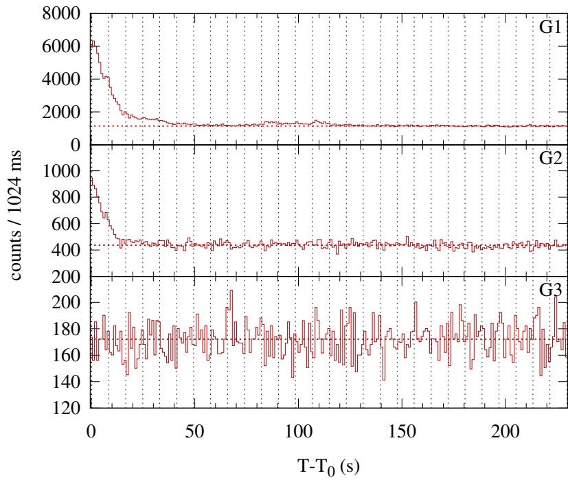
Konus-WIND S2 SOL2010-02-12T07:23 (C7.9) T_0 = 26597.710 s UT (07:23:17.710)
