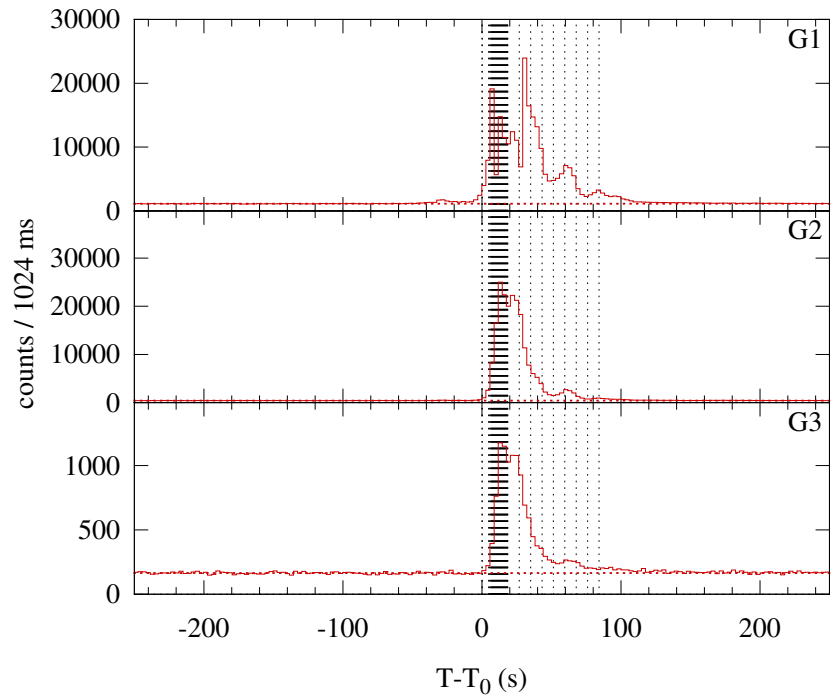
Konus-WIND S2 SOL2010-06-12T00:55 (M2.0) T_0 = 3332.314 s UT (00:55:32.314)
