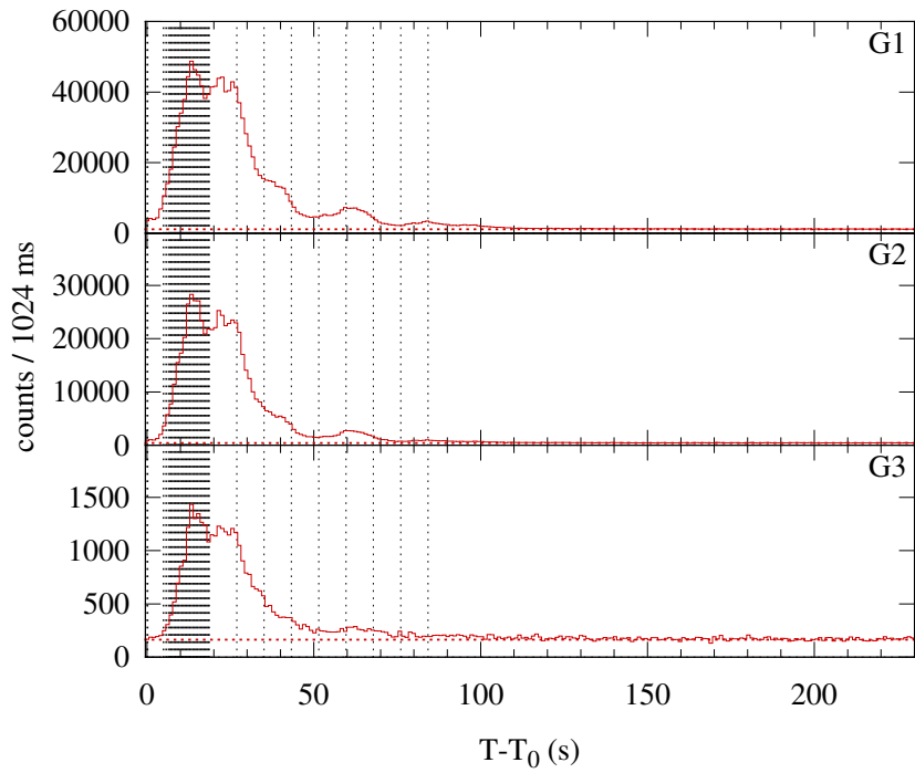
Konus-WIND S2 SOL2010-06-12T00:55 (M2.0) T_0 = 3332.314 s UT (00:55:32.314)
