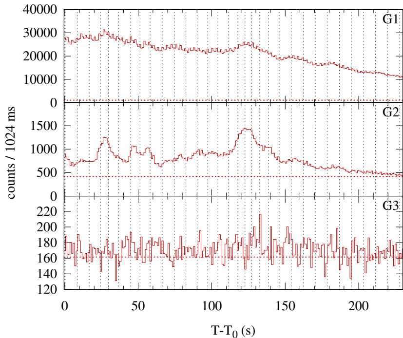
Konus-WIND S2 SOL2011-02-15T01:53 (X2.2) T_0 = 6788.473 s UT (01:53:08.473)
