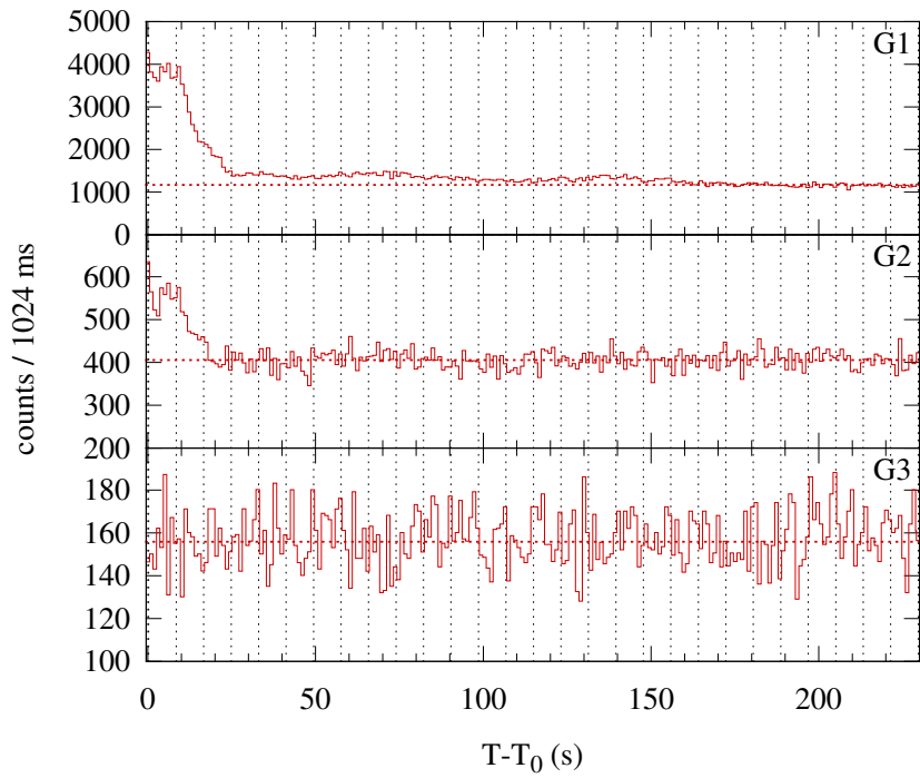
Konus-WIND S2 SOL2011-03-07T05:09 (M1.2) T_0 = 18599.922 s UT (05:09:59.922)
