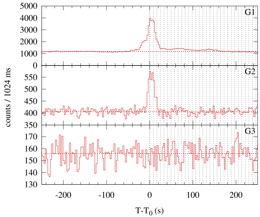
Konus-WIND S2 SOL2011-03-07T05:09 (M1.2) T_0 = 18599.922 s UT (05:09:59.922)
