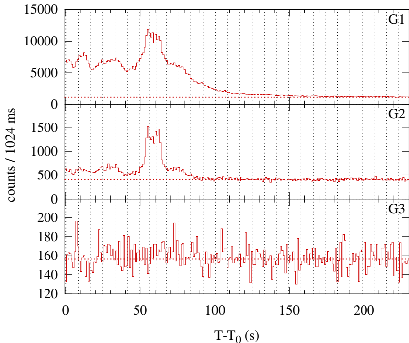
Konus-WIND S2 SOL2011-03-07T09:18 (M1.8) T_0 = 33485.85 s UT (09:18:05.85)
