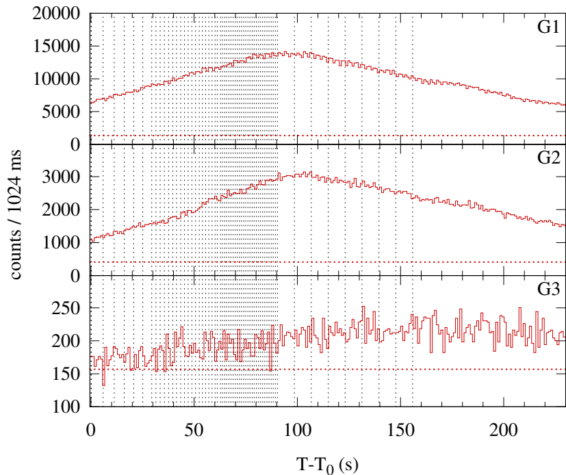
Konus-WIND S2 SOL2011-03-07T19:59 (M3.7) T 0 = 71959.180 s UT (19:59:19.180)
