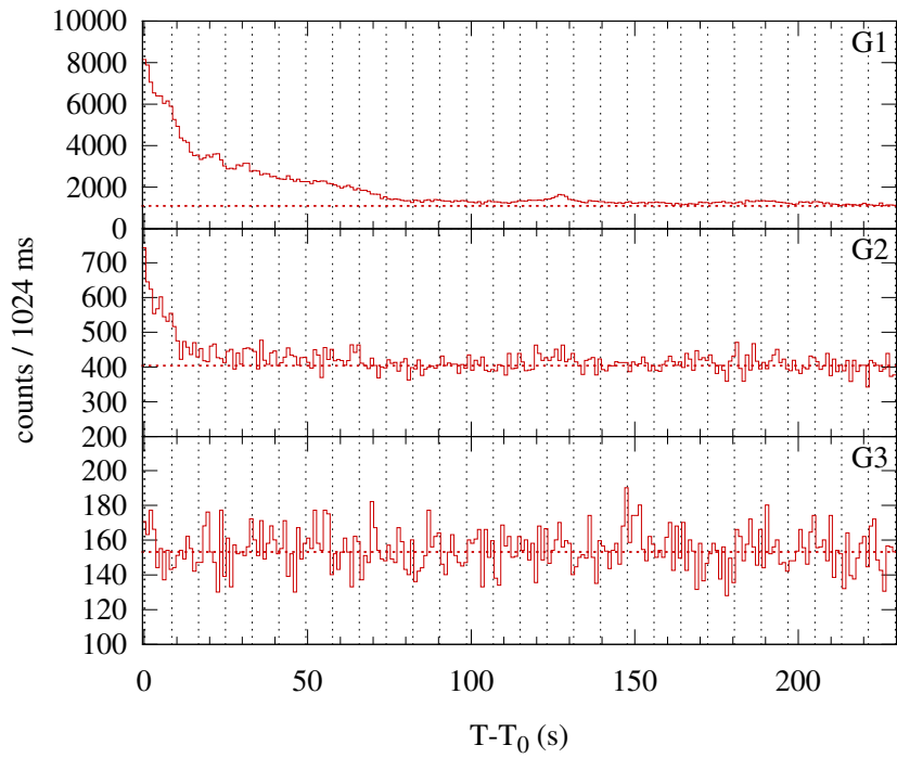
Konus-WIND S2 SOL2011-03-14T19:51 (M4.2) T_0 = 71484.357 s UT (19:51:24.357)
