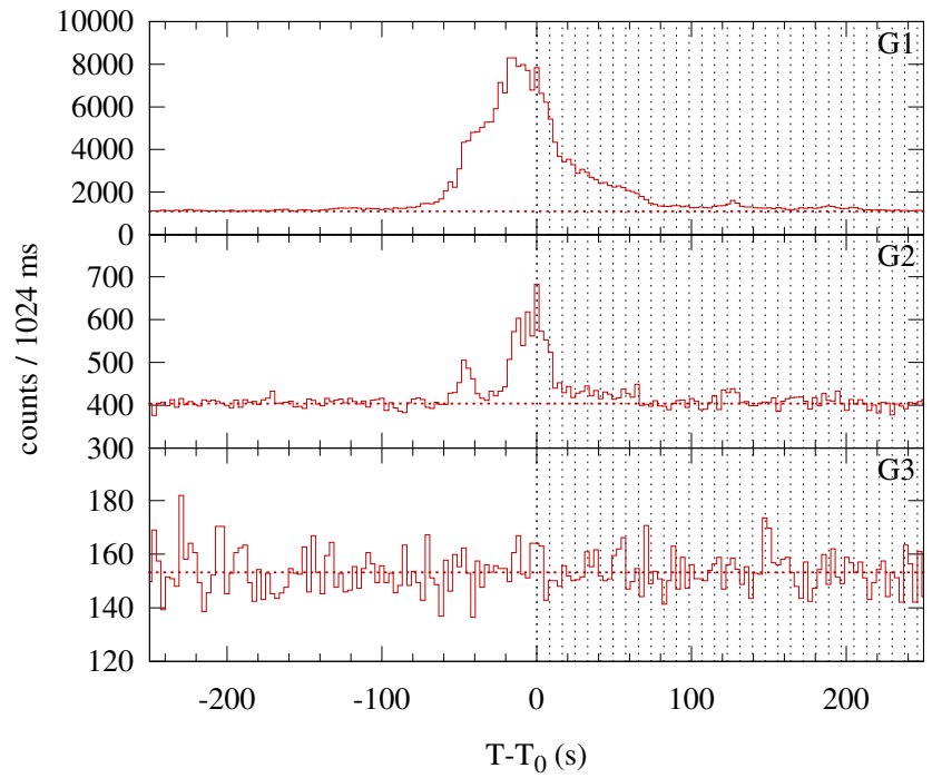
Konus-WIND S2 SOL2011-03-14T19:51 (M4.2) T_0 = 71484.357 s UT (19:51:24.357)
