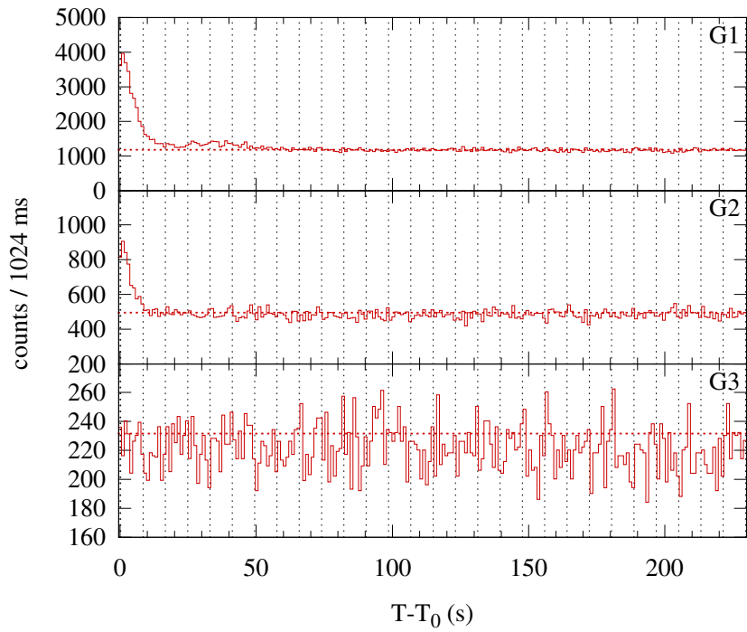
Konus-WIND S2 SOL2011-03-21T11:46 (C2.6) T_0 = 42378.799 s UT (11:46:18.799)
