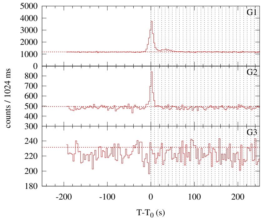
Konus-WIND S2 SOL2011-03-21T11:46 (C2.6) T_0 = 42378.799 s UT (11:46:18.799)
