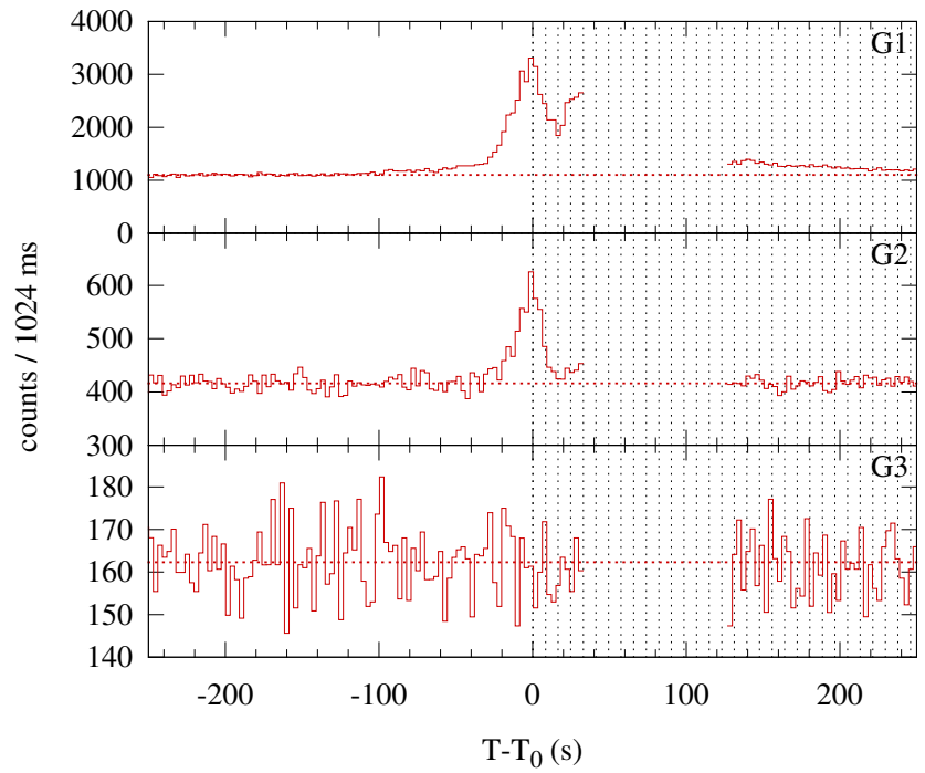
Konus-WIND S2 SOL2011-03-23T02:11 (M1.4) T 0 = 7902.595 s UT (02:11:42.595)
