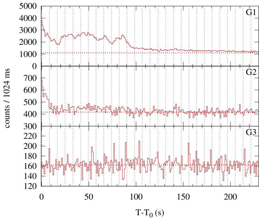
Konus-WIND S2 SOL2011-03-23T02:11 (M1.4) T 0 = 7902.595 s UT (02:11:42.595)
