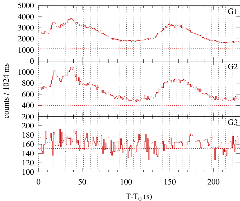
Konus-WIND S2 SOL2011-05-29T21:07 (C8.7) T_0 = 76051.482 s UT (21:07:31.482)
