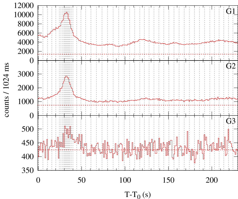
Konus-WIND S2 SOL2011-06-07T06:24 (M2.5) T_0 = 23094.454 s UT (06:24:54.454)
