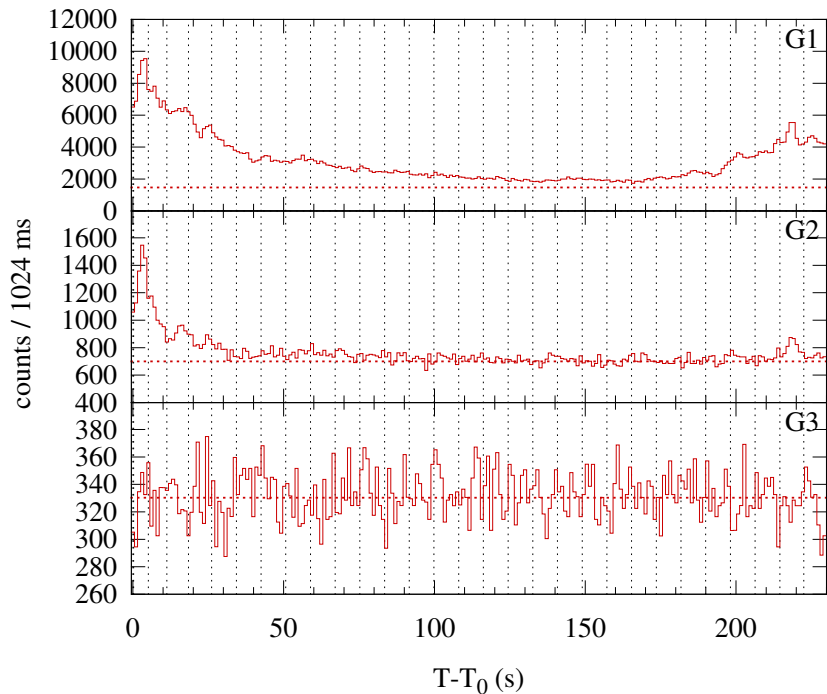
Konus-WIND S2 SOL2011-06-14T21:41 (M1.3) T 0 = 78089.578 s UT (21:41:29.578)
