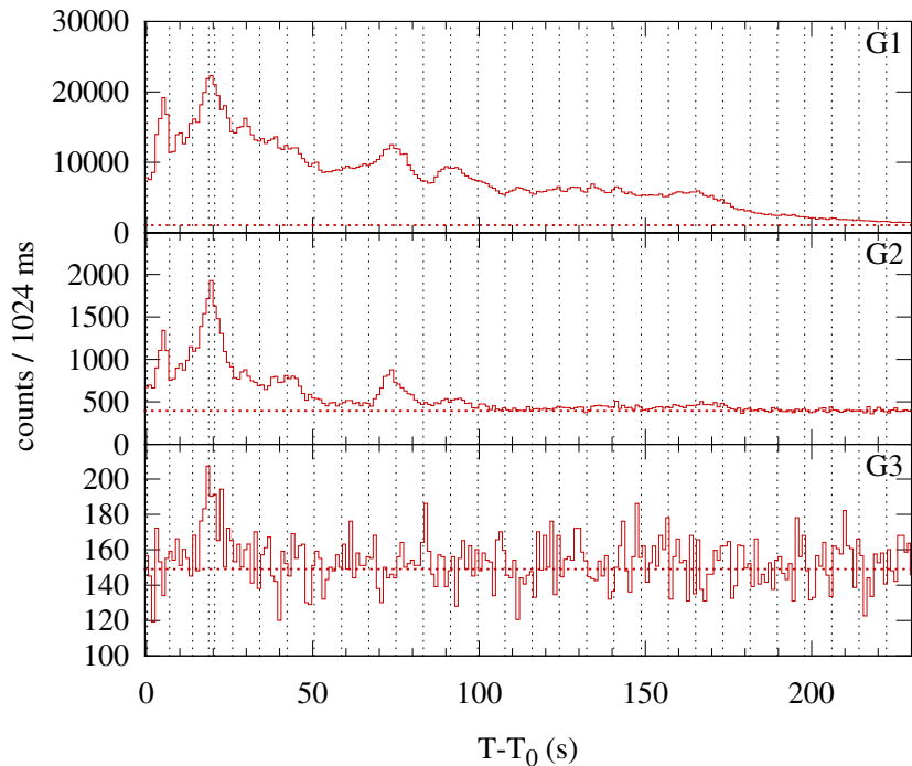
Konus-WIND S2 SOL2011-07-30T02:07 (M9.3) T 0 = 7651.497 s UT (02:07:31.497)
