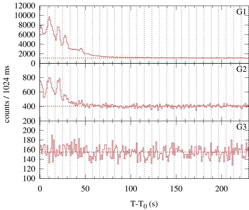
Konus-WIND S2 SOL2011-08-03T04:31 (M1.7) T_0 = 16261.758 s UT (04:31:01.758)
