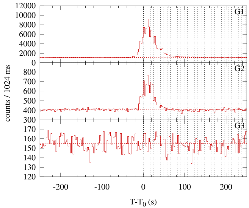
Konus-WIND S2 SOL2011-08-03T04:31 (M1.7) T_0 = 16261.758 s UT (04:31:01.758)
