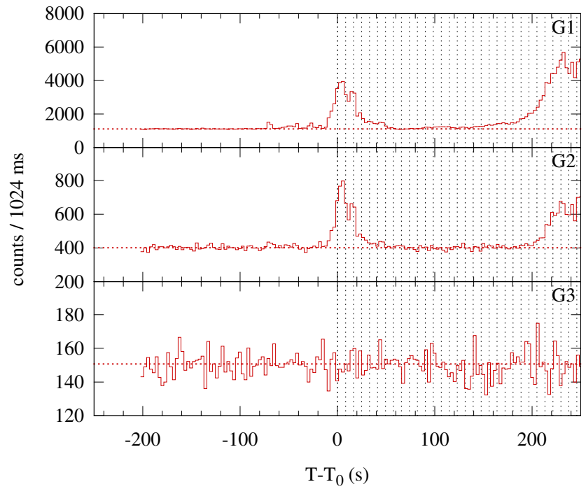
Konus-WIND S2 SOL2011-08-04T03:45 (M9.3) T_0 = 13523.117 s UT (03:45:23.117)
