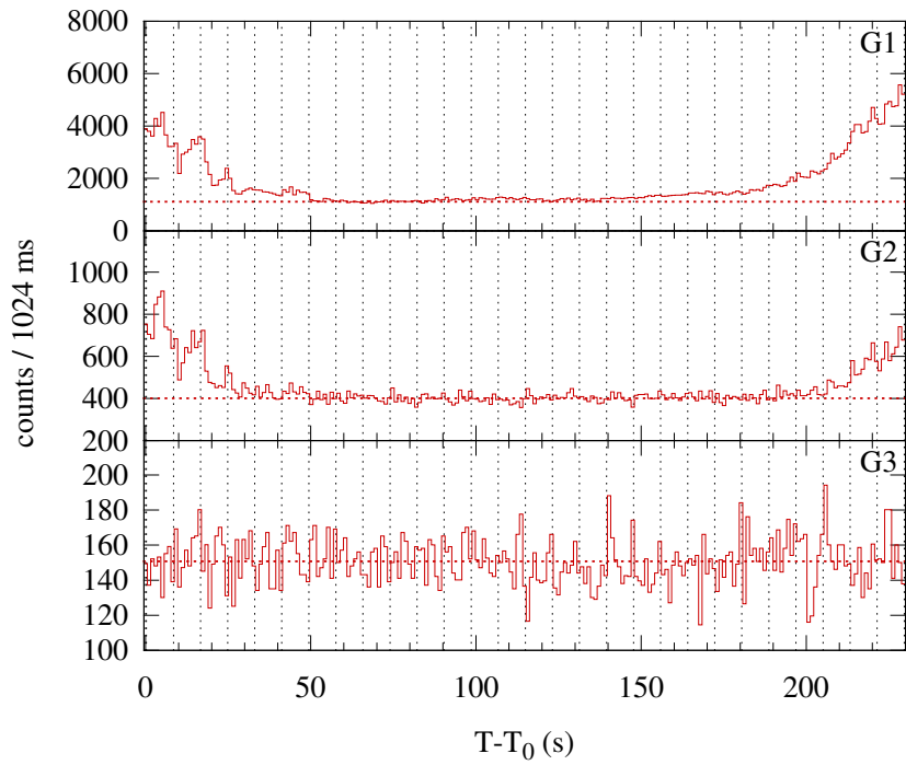
Konus-WIND S2 SOL2011-08-04T03:45 (M9.3) T_0 = 13523.117 s UT (03:45:23.117)
