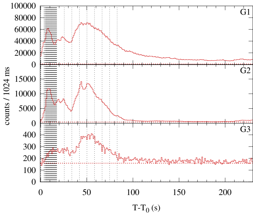
Konus-WIND S2 SOL2011-09-06T22:18 (X2.1) T_0 = 80285.187 s UT (22:18:05.187)
