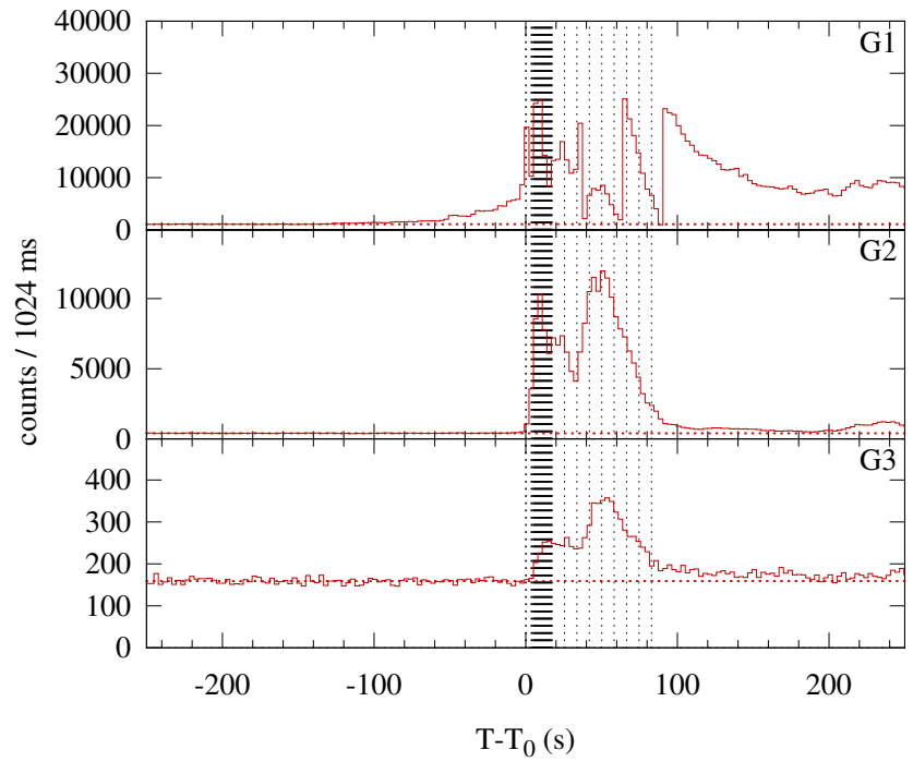
Konus-WIND S2 SOL2011-09-06T22:18 (X2.1) T_0 = 80285.187 s UT (22:18:05.187)
