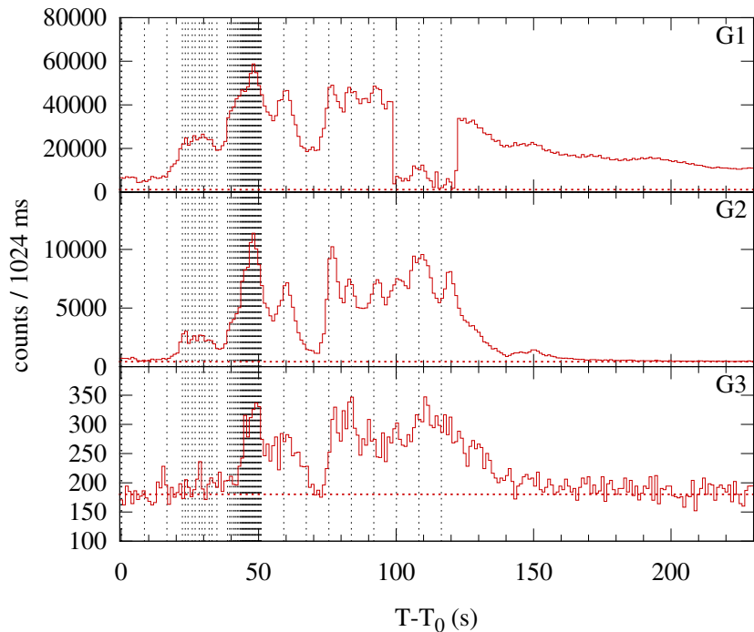
Konus-WIND S2 SOL2011-09-07T22:35 (X1.8) T_0 = 81326.331 s UT (22:35:26.331)
