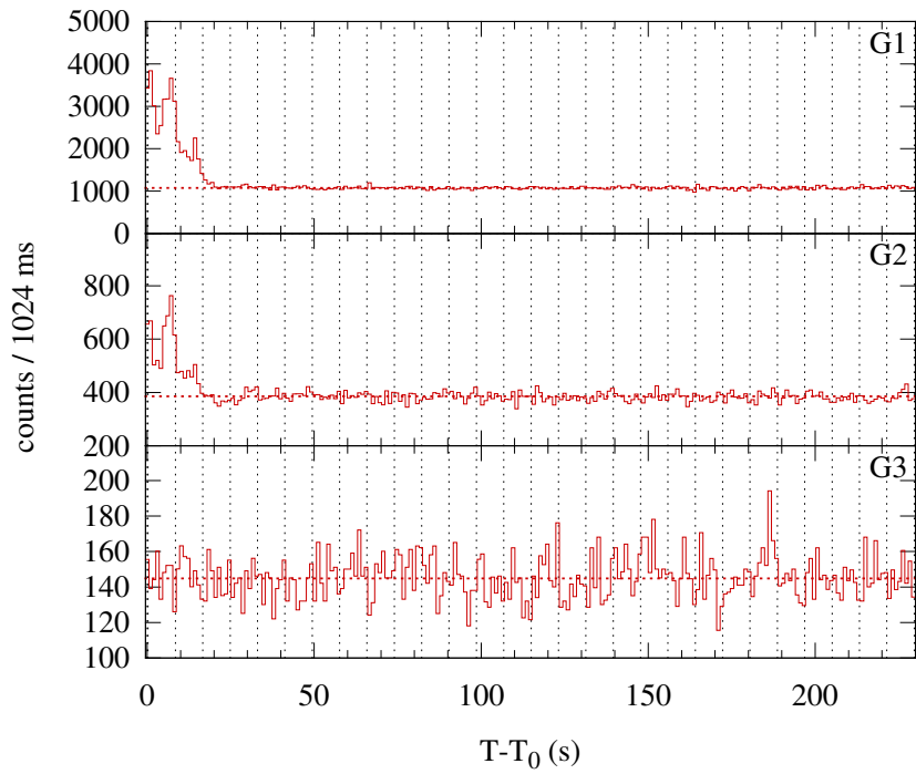
Konus-WIND S2 SOL2011-09-20T06:48 (C2.0) T 0 = 24486.21 s UT (06:48:06.21)
