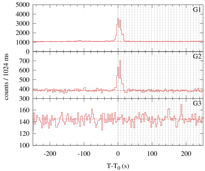
Konus-WIND S2 SOL2011-09-20T06:48 (C2.0) T 0 = 24486.21 s UT (06:48:06.21)
