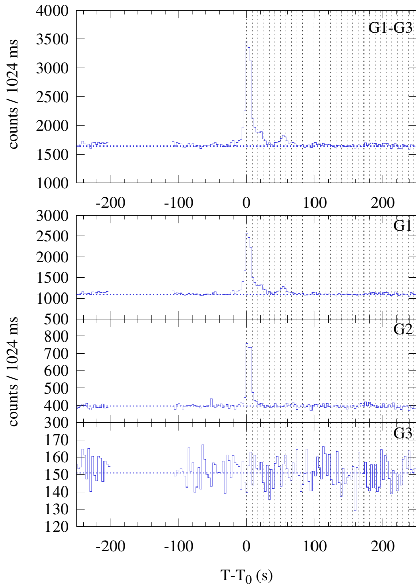
Konus-WIND S2 SOL2011-09-22T04:27 (C6.6) T_0 = 16061.276 s UT (04:27:41.276)
