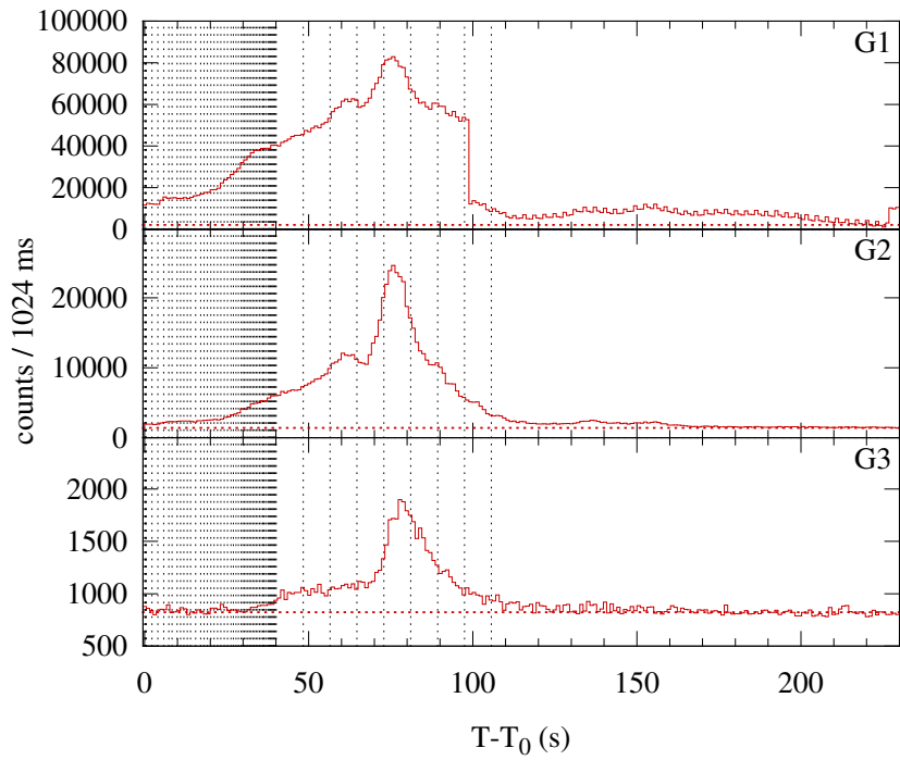
Konus-WIND S2 SOL2011-09-24T09:35 (X1.9) T 0 = 34503.350 s UT (09:35:03.350)
