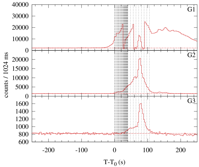
Konus-WIND S2 SOL2011-09-24T09:35 (X1.9) T 0 = 34503.350 s UT (09:35:03.350)
