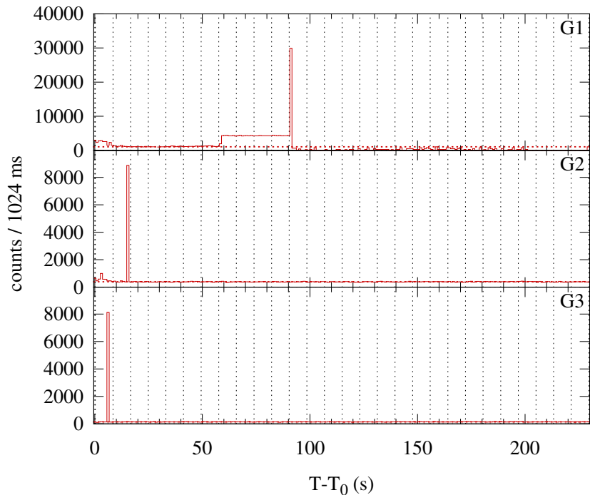
Konus-WIND S2 SOL2011-10-19T18:46 (C3.4) T 0 = 67615.565 s UT (18:46:55.565)
