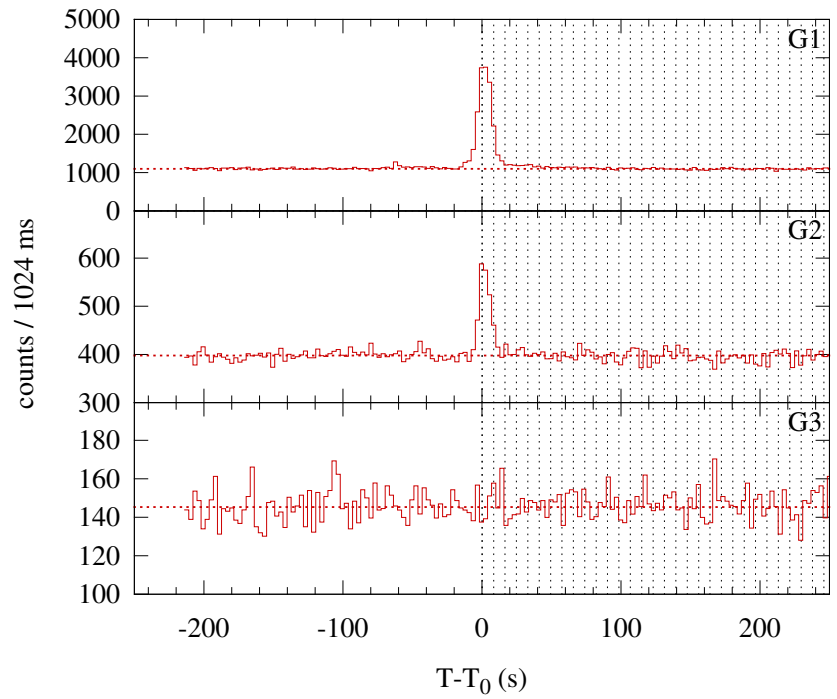
Konus-WIND S2 SOL2011-12-05T15:17 (C4.7) T 0 = 55021.232 s UT (15:17:01.232)
