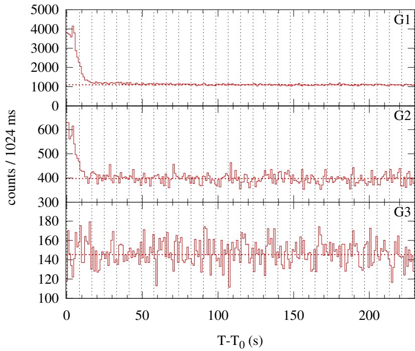
Konus-WIND S2 SOL2011-12-05T15:17 (C4.7) T 0 = 55021.232 s UT (15:17:01.232)
