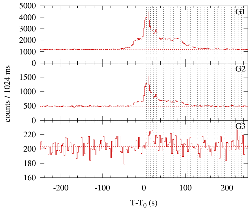
Konus-WIND S2 SOL2011-12-25T20:26 (C7.7) T_0 = 73610.583 s UT (20:26:50.583)
