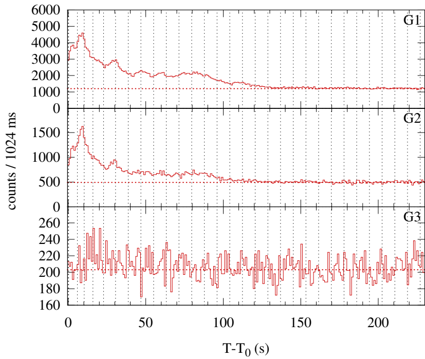
Konus-WIND S2 SOL2011-12-25T20:26 (C7.7) T_0 = 73610.583 s UT (20:26:50.583)
