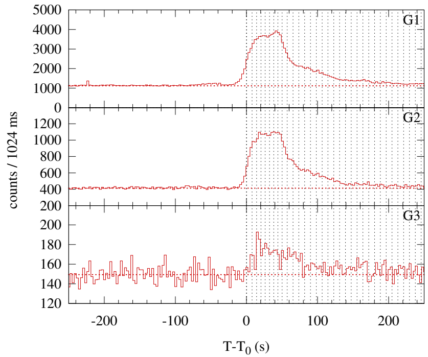
Konus-WIND S2 SOL2011-12-27T04:16 (C8.9) T 0 = 15360.966 s UT (04:16:00.966)
