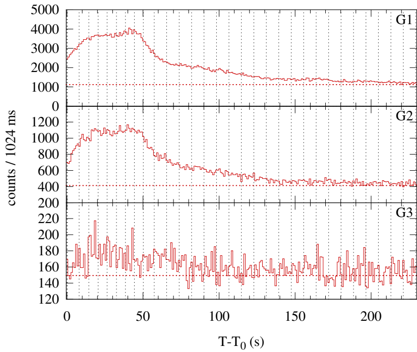
Konus-WIND S2 SOL2011-12-27T04:16 (C8.9) T 0 = 15360.966 s UT (04:16:00.966)
