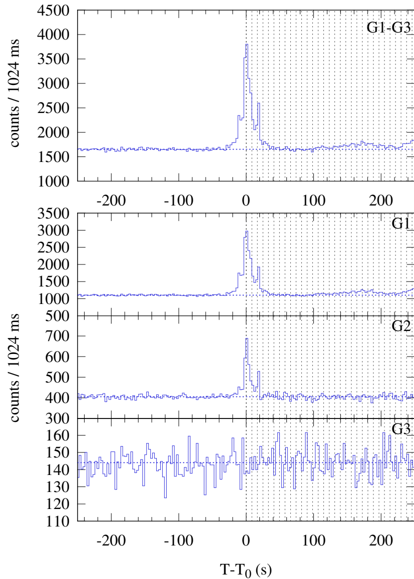
Konus-WIND S2 SOL2011-12-31T16:19 (M1.5) T_0 = 58783.680 s UT (16:19:43.680)
