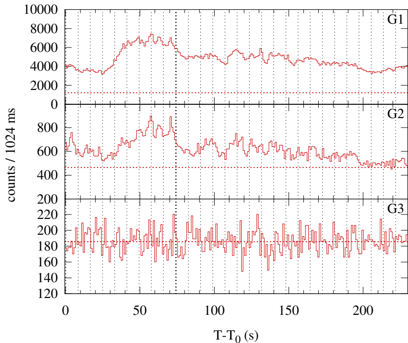
Konus-WIND S2 SOL2012-03-05T03:33 (X1.1) T 0 = 12821.782 s UT (03:33:41.782)
