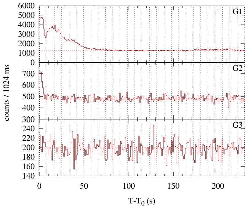
Konus-WIND S2 SOL2012-03-06T21:05 (M1.3) T_0 = 75935.680 s UT (21:05:35.680)
