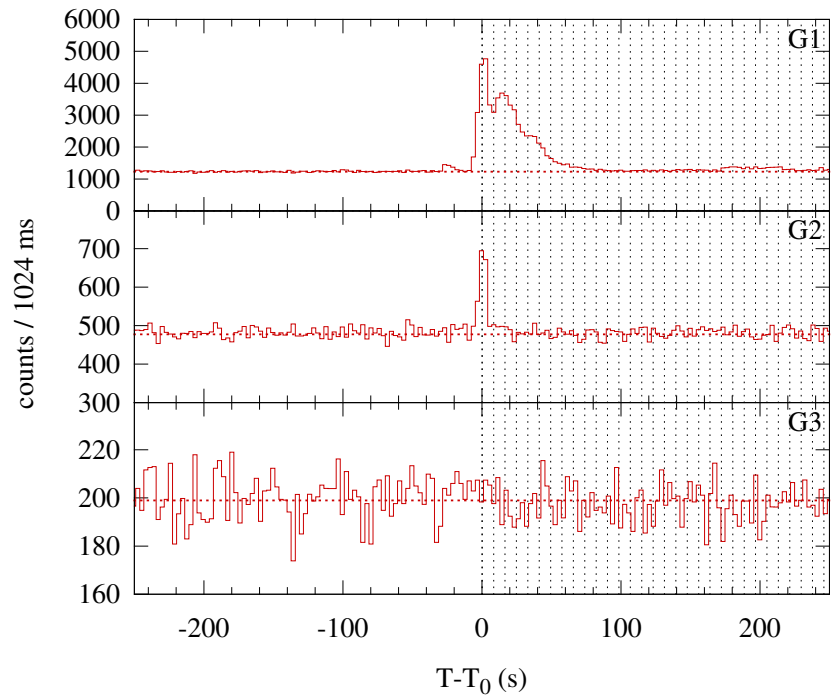
Konus-WIND S2 SOL2012-03-06T21:05 (M1.3) T_0 = 75935.680 s UT (21:05:35.680)
