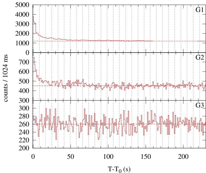
Konus-WIND S2 SOL2012-03-17T20:36 (M1.3) T 0 = 74201.770 s UT (20:36:41.770)
